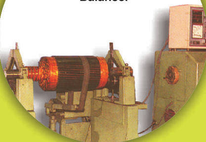
Electronic Two - Axle Balancer
